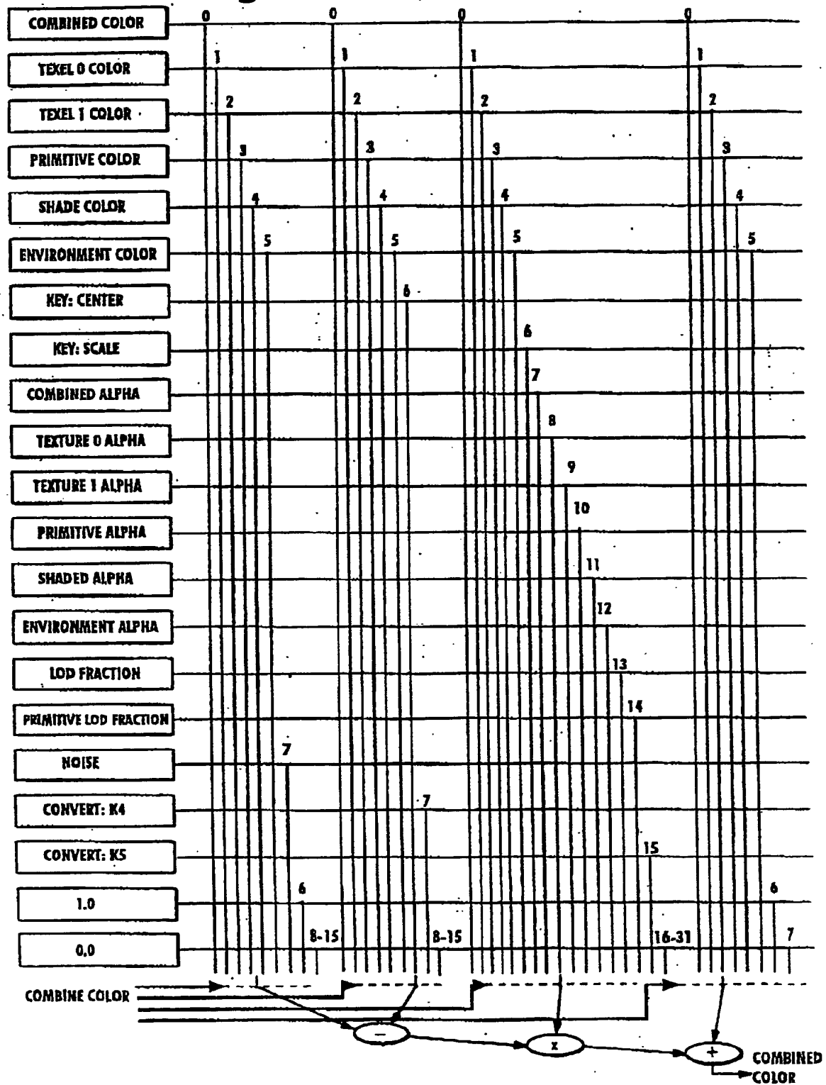
Fig. 27 RGB COLOR COMBINER EXAMPLE INPUT SELECTION
